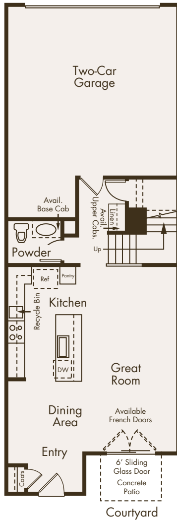
FIRST FLOOR
